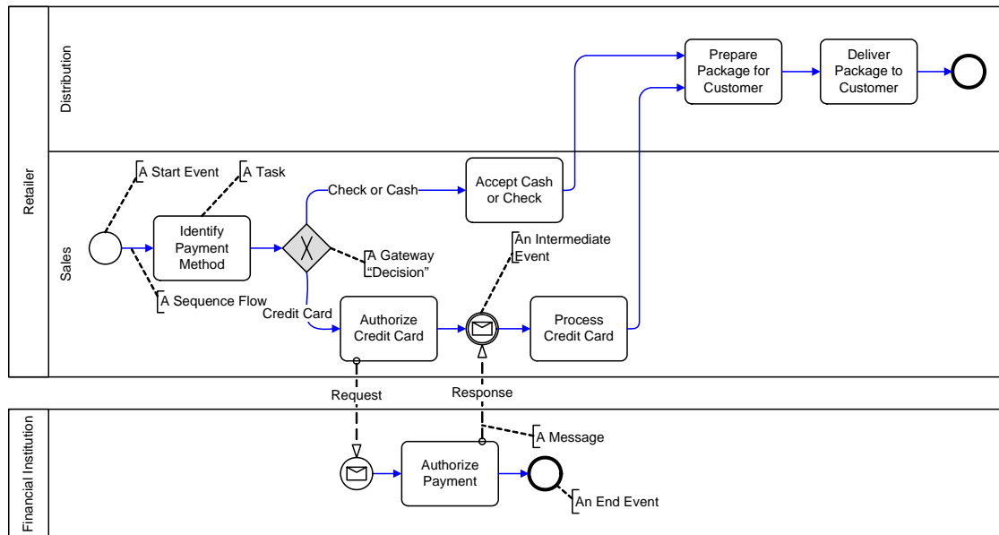
Figure 1: BPMN model of a payment process
