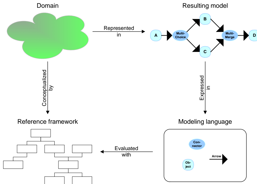
Figure 2: Relations between domain, reference framework, modeling language and model
