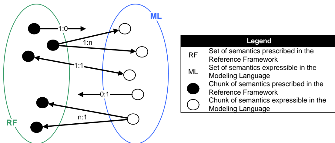
Figure 3: Framework for language evaluation
