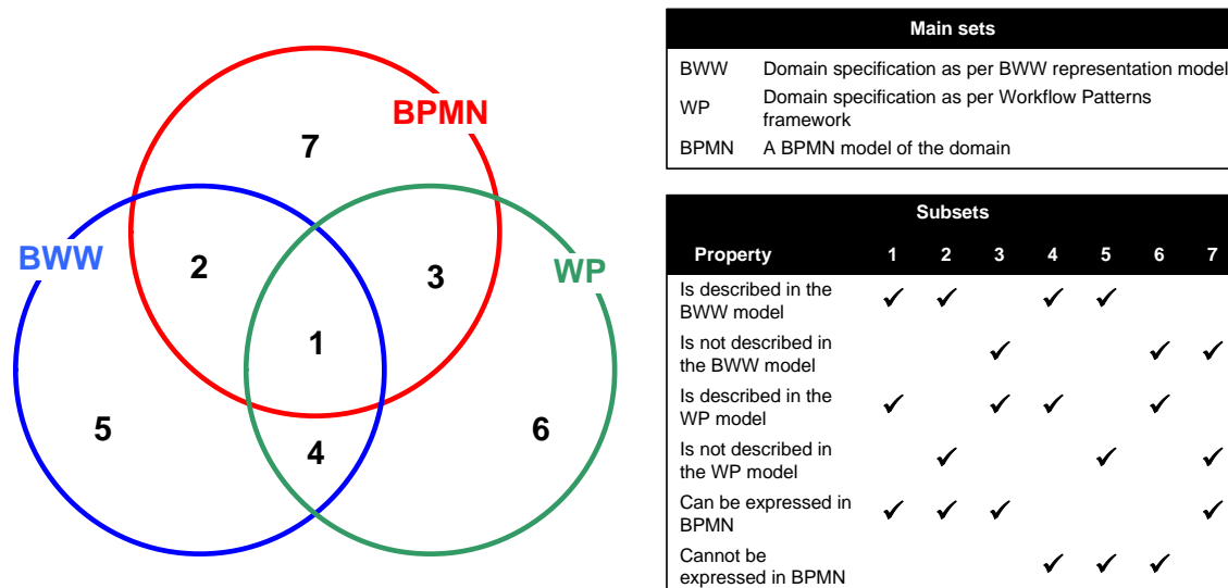
Figure 4: Set model showing relationships between reference frameworks and modeling language
