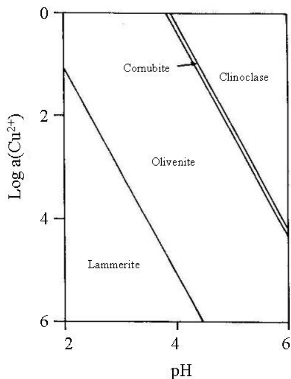
Figure 1 Phase relationship of some of the basic copper arsenate minerals (after Williams, 1990)
