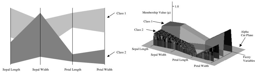
Fig. 3. (Left) Illustration of 2D method developed by Holve and Berthold, for representing multidimensional fuzzy rules using fuzzy parallel coordinates [2]. Two rules are illustrated from their Iris data example. (Right) Visualisation of the Iris data with lit and textured surfaces showing the same Iris data. Note how the alpha cutting of the membership function for Rule 2 on the Petal Length dimension is easily perceived.
