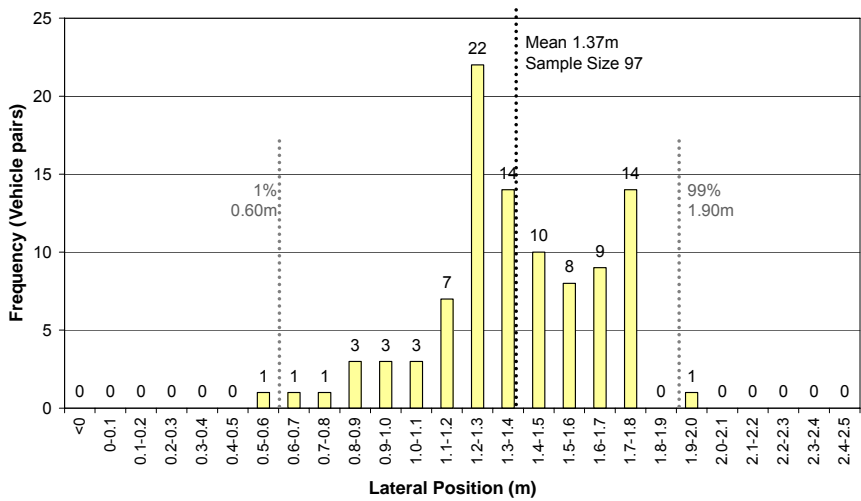
Figure 11: Lateral position passenger car: Semi-trailer (any lane)
