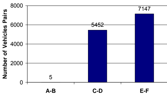
Figure 4: Bar graph showing number of vehicles arriving in each LOS category
