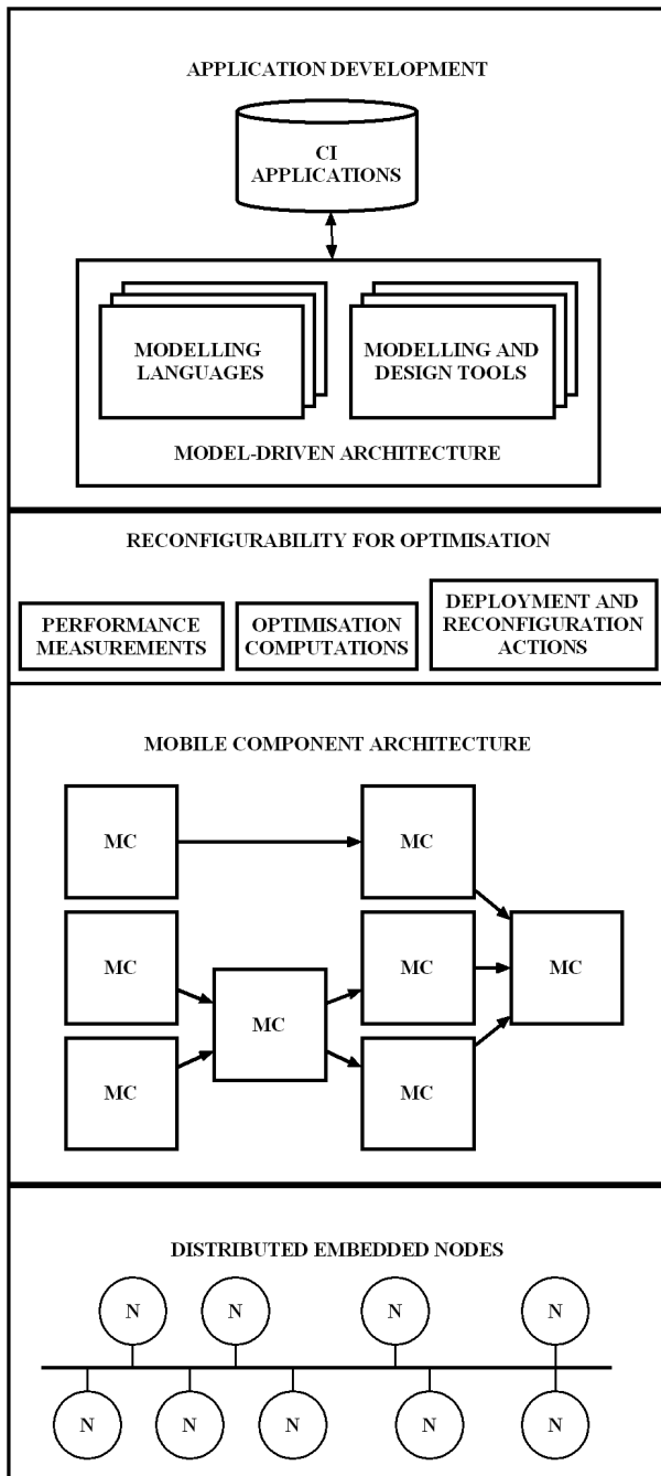
Figure 2. Proposed Framework
