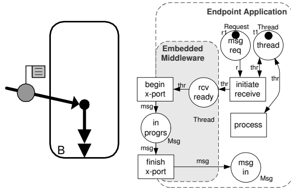
(a) Notation, non- (b) CPN of non-blocking receive.
