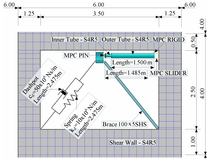
Fig.5 - Details of hybrid friction-VE damper.
