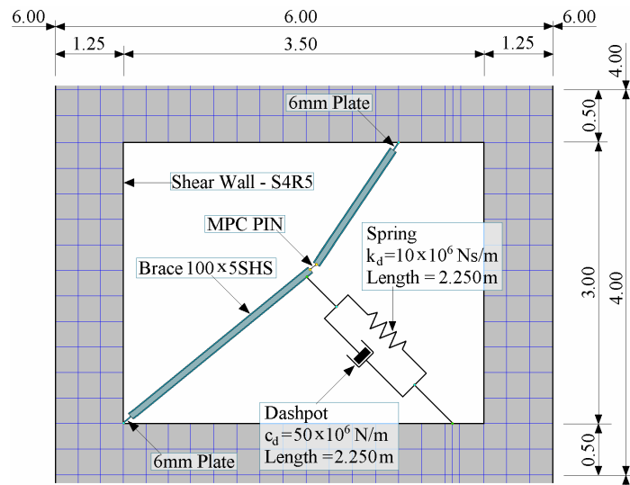
Fig.8 - Details of lower toggle VE damper.
