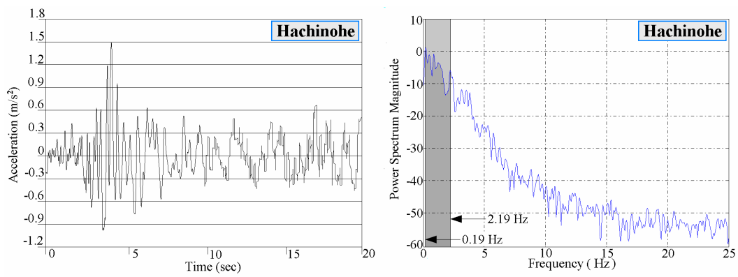
Fig.10 - Hachinohe earthquake record and its dominant frequencies.
