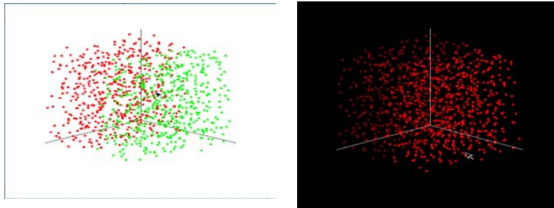
Fig.2. (Left) Different colours used to indicate membership of different membership function terms. In this case, the red indicates slow motion, while the green indicates fast motion. (Right) Intensity difference as an indication of the membership degree for a fuzzy membership function Hot.
