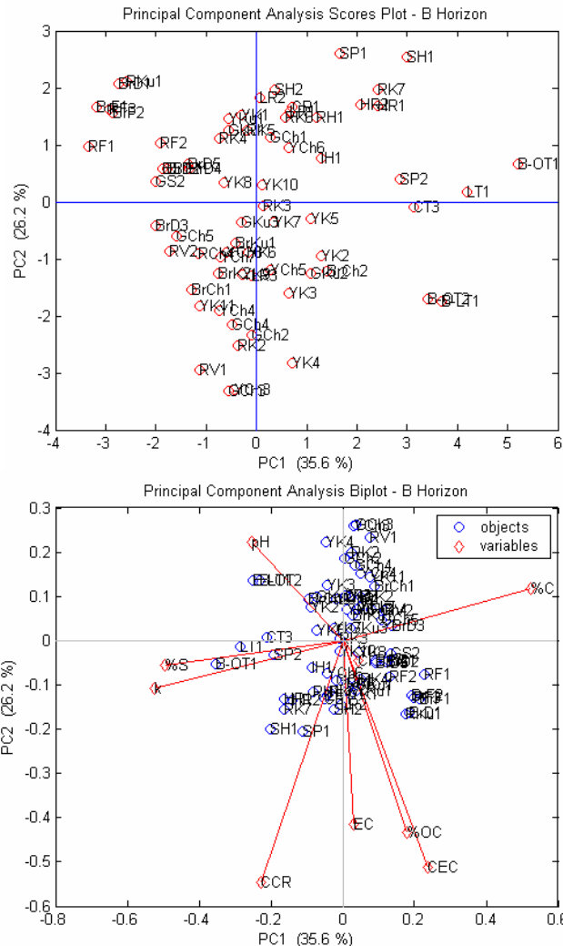
Figure 2: Scores and biplot for PCA Analysis
