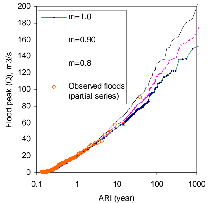
Figure 3. Effects of changing m on flood peaks for Boggy River catchment.
