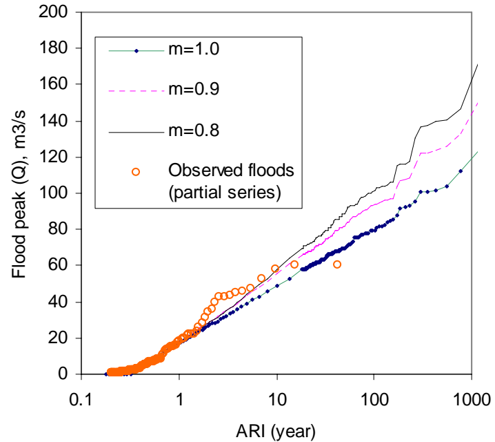
Figure 2. Effects of changing m on flood peaks for Avoca River catchment.
