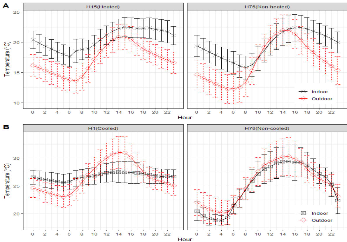
Figure 3(A) Daily patterns in hourly mean indoor and outdoor temperatures during cool season in AC (heated) (H15) and non-AC (non-heated) (H76) houses. (B) Daily patterns in hourly mean indoor and outdoor temperatures during the warm season in a cooled (H1) and not cooled (H76) houses. Each panel represents one house
