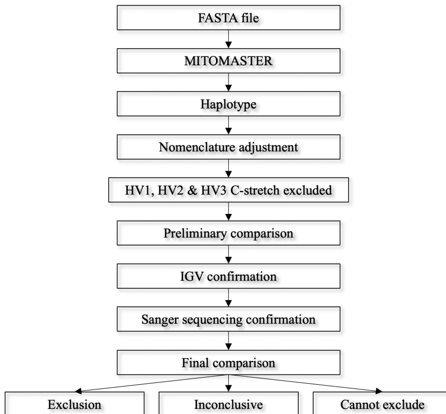
FIGURE 1 Overview of the interpretation process. The process undertaken to identify mtDNA haplotypes for each participant and perform sequence comparisons. Haplotypes are generated using MITOMASTER, then altered to align with existing interpretation guidelines. Variants were confirmed through SS before undertaking final comparison
