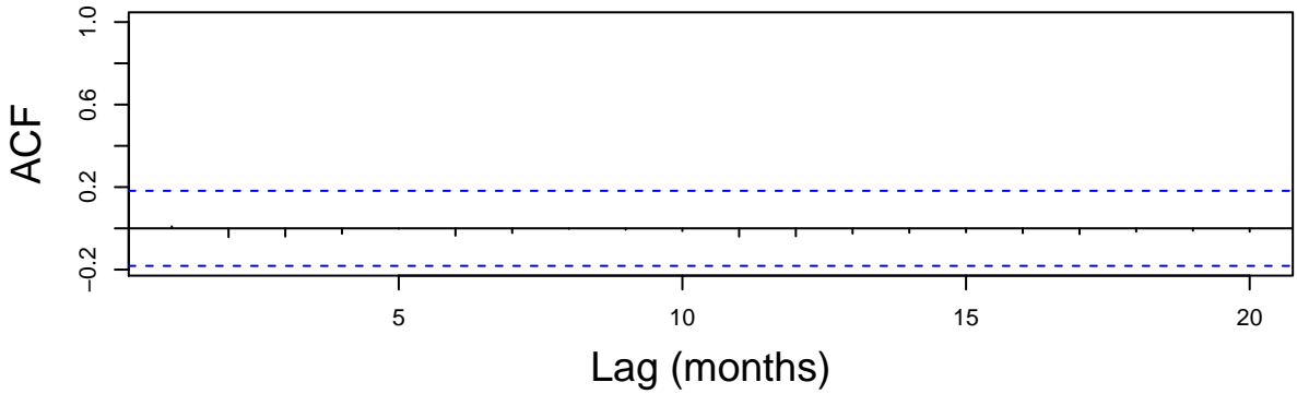
Auto-correlation function for residuals of DLM
