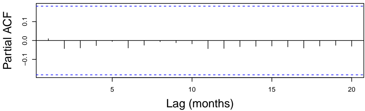
Partial auto-correlation function for residuals of DLM
