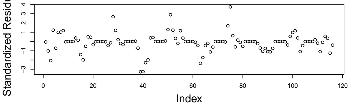
Scatter plot for residuals of DLM
