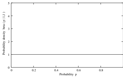
(a) Uniform PDF \text{beta}(p | 1, 1)
