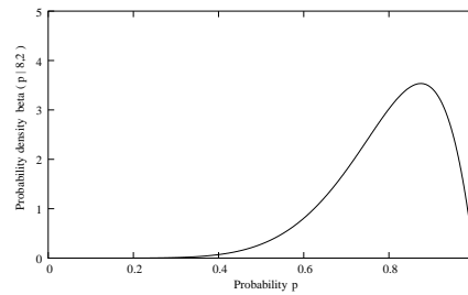
(b) PDF \text{beta}(p | 8, 2)
